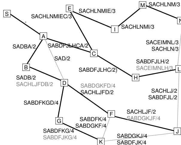
Figure 4: Final Result of Backup Multicast Tree Construction
