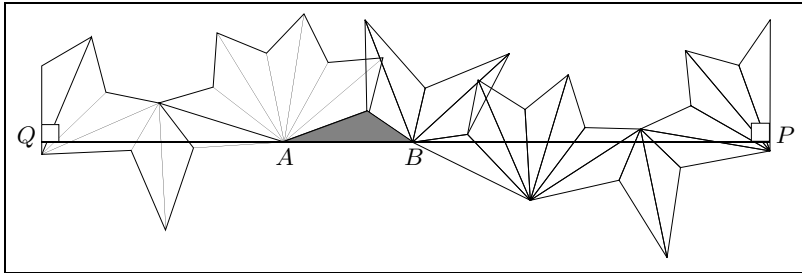
Fig. 10: Degenerate path along the basis
