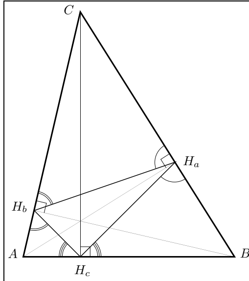
Fig. 2: Orthoptic triangle
