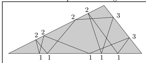
Fig. 4: Periodic billiard path corresponding to the code (1, 3, 2, 1, 2, 1, 2, 1, 3, 1, 2)
