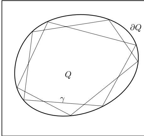
Fig. 1: A periodic billiard trajectory \gamma in Q with 9 reflections and winding number 2.
