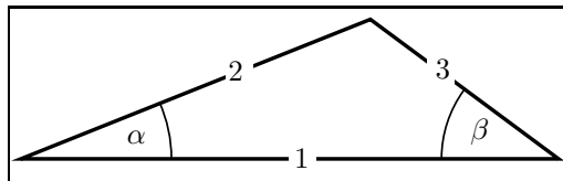
Fig. 3: Angles and sides in an obtuse triangle
