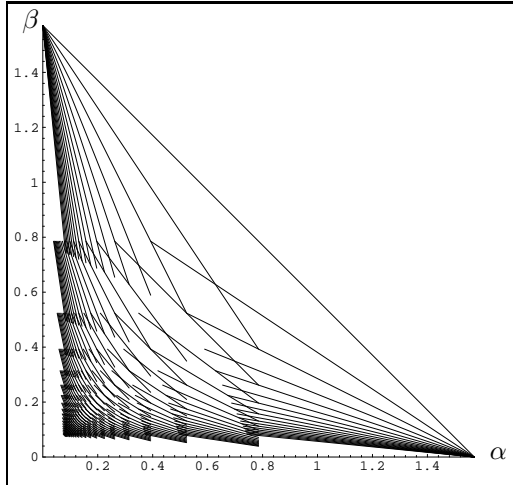
Fig. 6: Perpendicular trajectories
