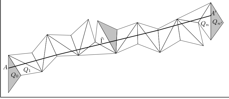
Fig. 5: Straightened billiard trajectory
