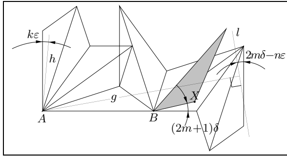
Fig. 14: Limiting situation
