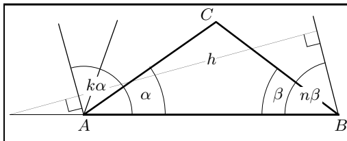
Fig. 7: Perpendicular trajectories
