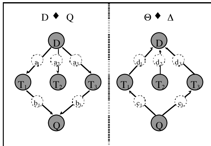
Figure 1 : Representation of the PAS for the DQ and QD interpretations of relevance
