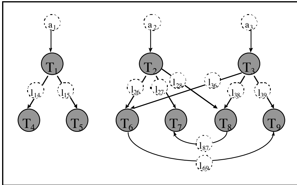
Figure 3 : Example of a PAS for query expansion
