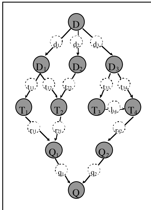
Figure 2 : Example of a PAS for modeling IR
